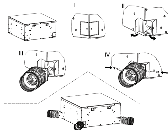
» Fig.17 FWH-A 02-03-04
