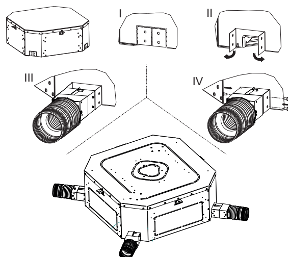
» Fig.18 FWH-A 06-07-08
