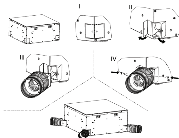
» Fig.17 FWH-A 02-03-04
