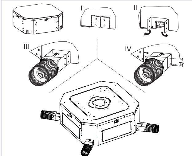
» Fig.18 FWH-A 06-07-08
