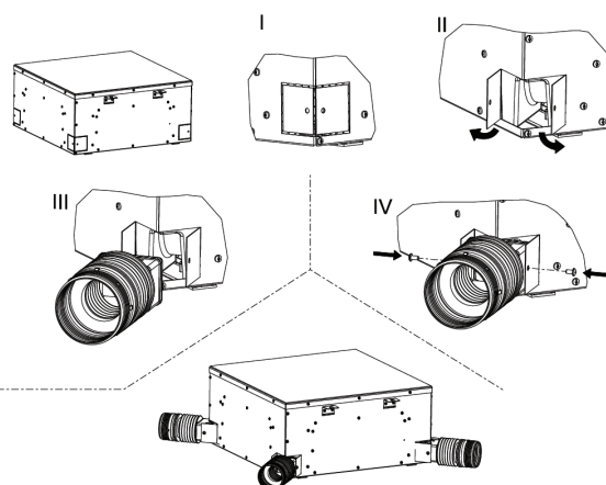
» Fig.17 FWH-A 02-03-04
